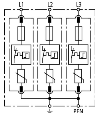
Basic circuit diagram DG M TNC CI 275
