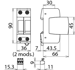
Dimension drawing DG M TN CI 275 FM
