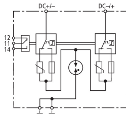
Basic circuit diagram DCB YPV SCI 1500 FM
